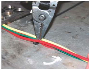
Cuts cable ties from bundled wires without damaging insulation
